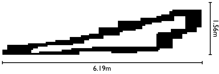
Cross-section A
